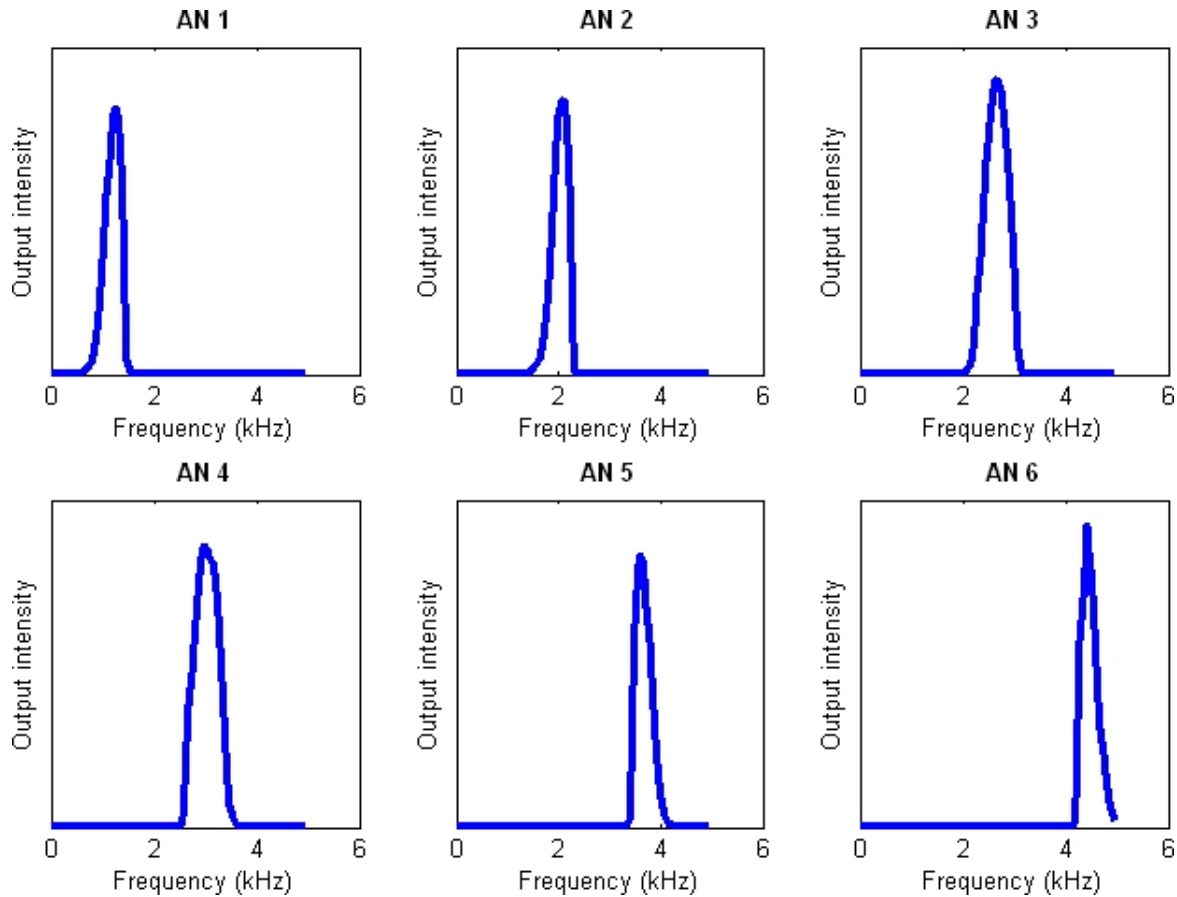
Figure 5: Tuning curves from neural network. The artificial neurons (ANs) are selective for frequencies where response intensity is greater than zero. The peak of the curves gives the best frequency (BF) of the AN. These graphs do not describe the artificial neurons in the temporal domain.
