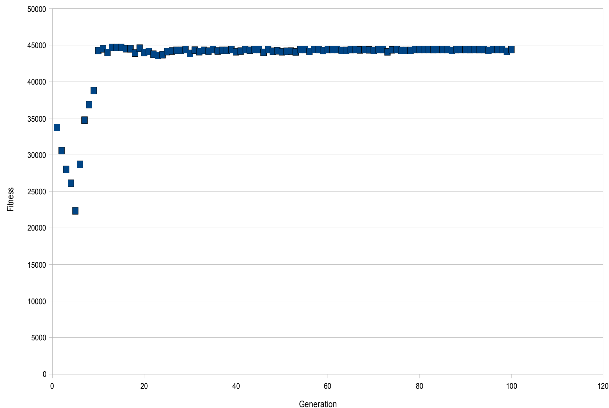
Average Fitness by Generation
