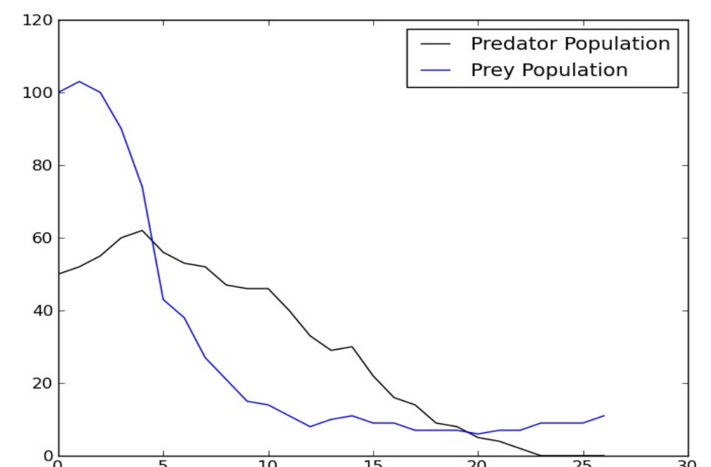
Figure 2. Behavioral Model
