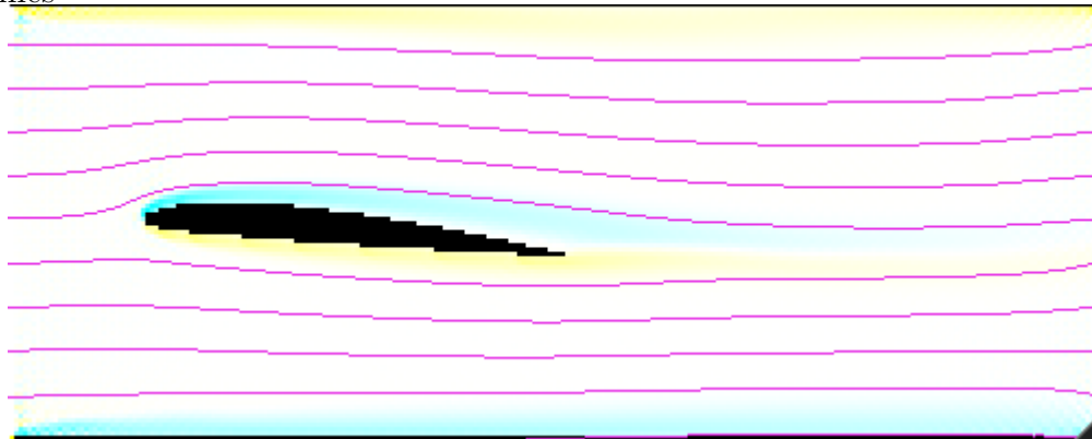
Figure 5: In process wind tunnel test visualized using vorticity and streamlines
