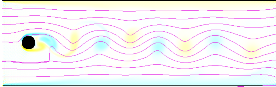
Figure 4: In process flow past a cylinder test visualized using vorticity and streamlines demonstrating the Kármán vortex street
