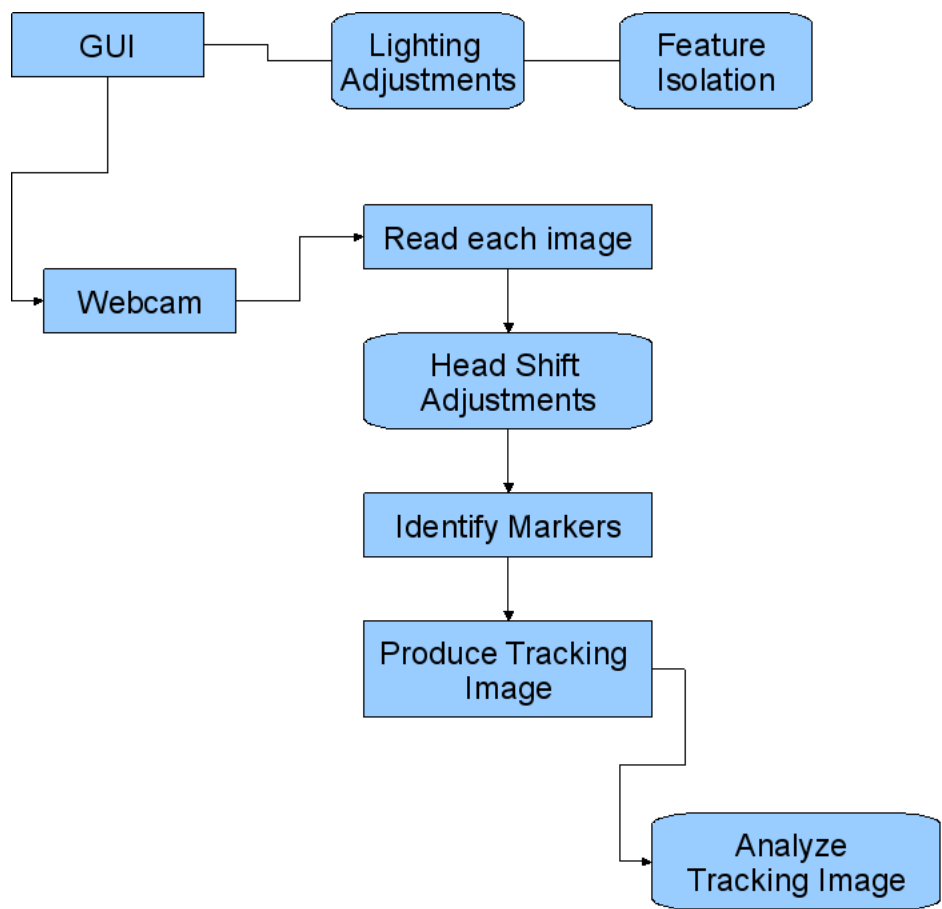
Figure 2: The basic structure of the program.
