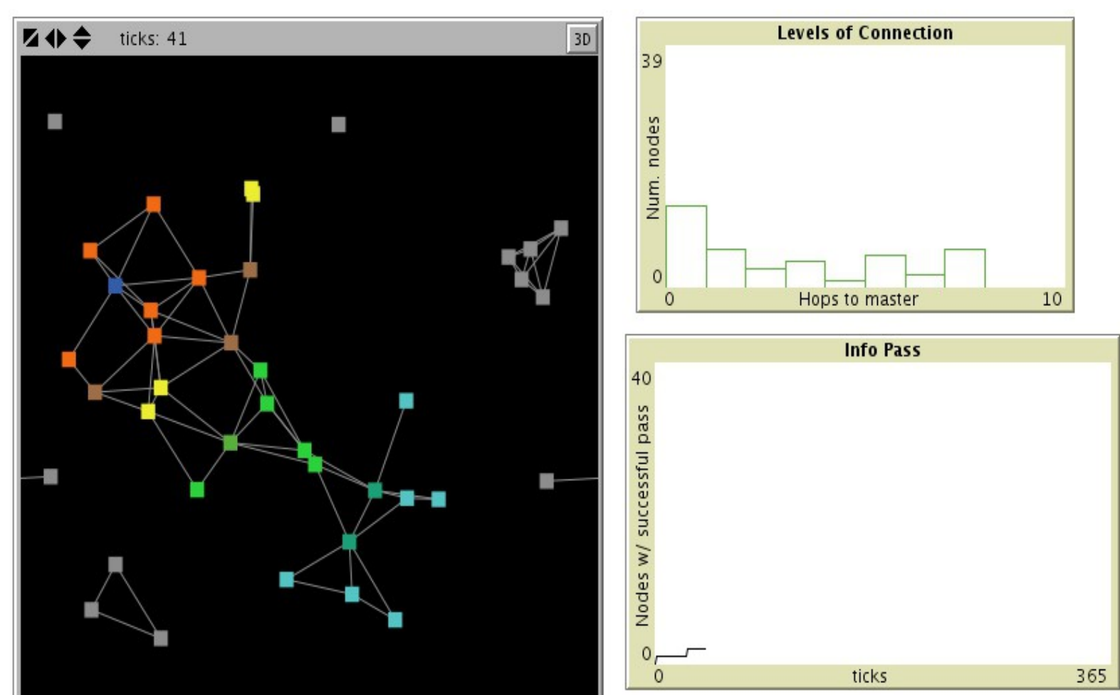
Figure 2: The NetLogo model. Left: visualization of levels of connection to the master-node. Right top: histogram of nodes with different levels of connection. Right bottom: Number of nodes with successful information passing after 41 ticks.
